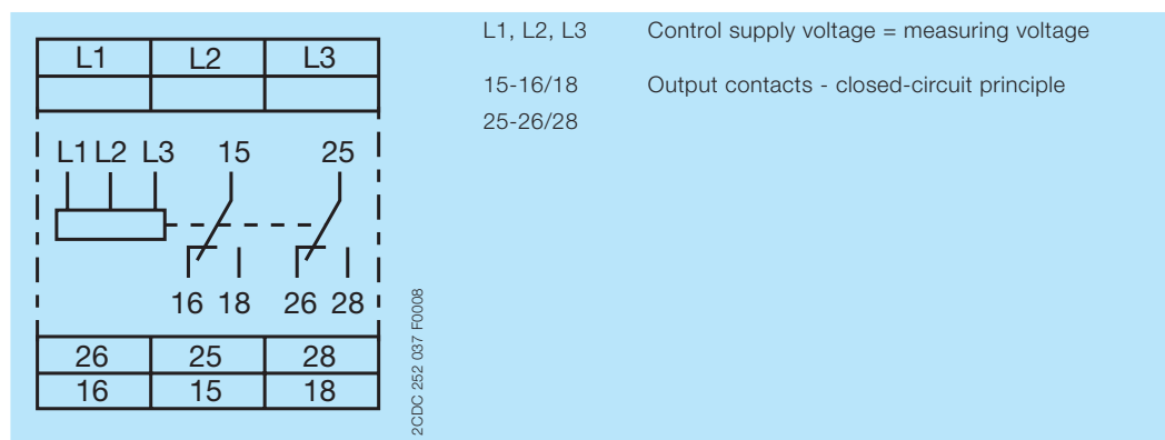
Connection diagram CM-MPS.43
