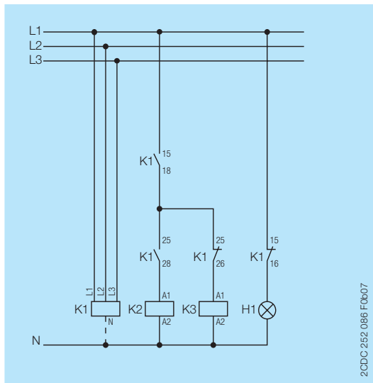
Control circuit diagram (K1 = CM-MPS.x3)
