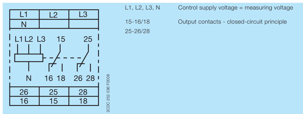
Connection diagram CM-MPS.23
